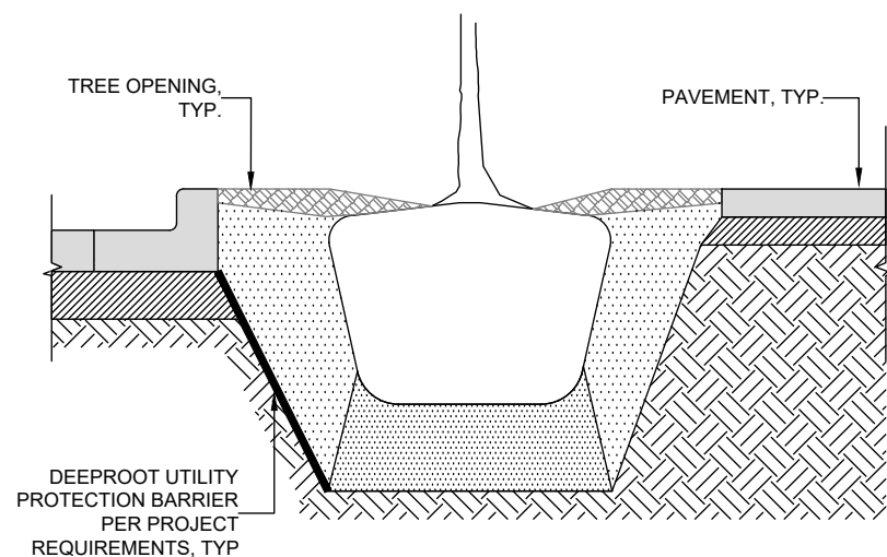
○ DEEPROOT UTILITY PROTECTION BARRIER - ROADWAY APPLICATION NOT TO SCALE
