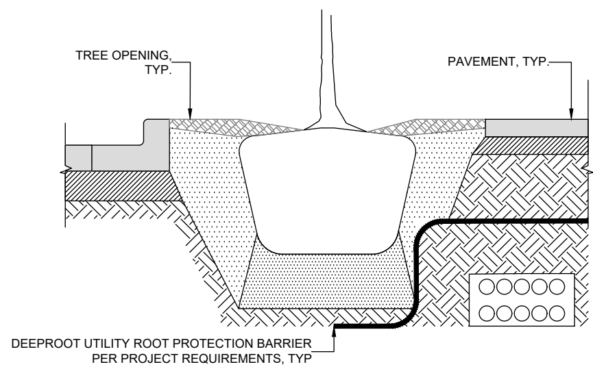
○ DEEPROOT UTILITY ROOT PROTECTION BARRIER-DUCT BANK APPLICATION NOT TO SCALE
