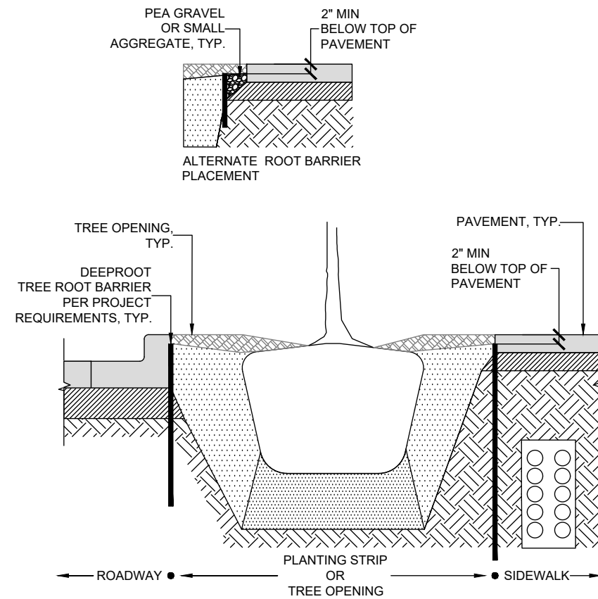
DEEPROOT TREE ROOT BARRIER - UB 36-2 AND UB 48-2 NOT TO SCALE
