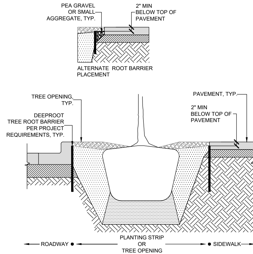
DEEPROOT TREE ROOT BARRIER - UB 24-2 NOT TO SCALE
