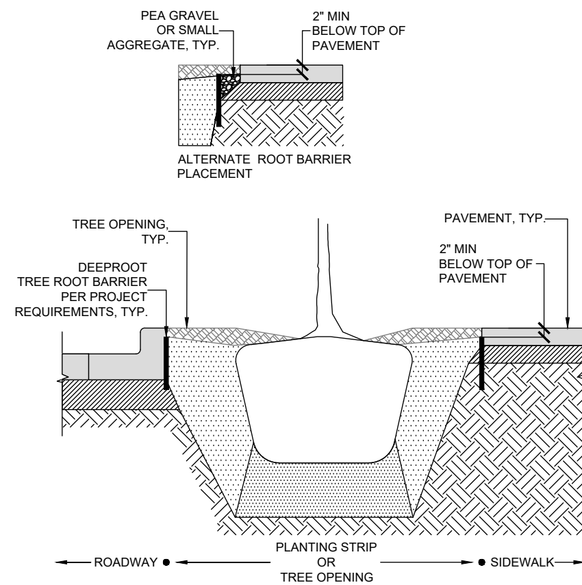
DEEPROOT TREE ROOT BARRIER - UB 12-2 NOT TO SCALE
